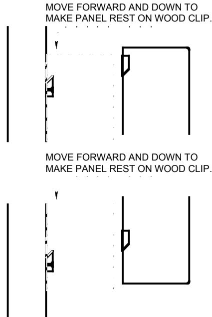
3 MOUNTING DETAIL 03.00 Scale: 1:10
