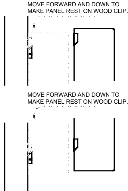
3 MOUNTING DETAIL 04.00 Scale: 1:10
