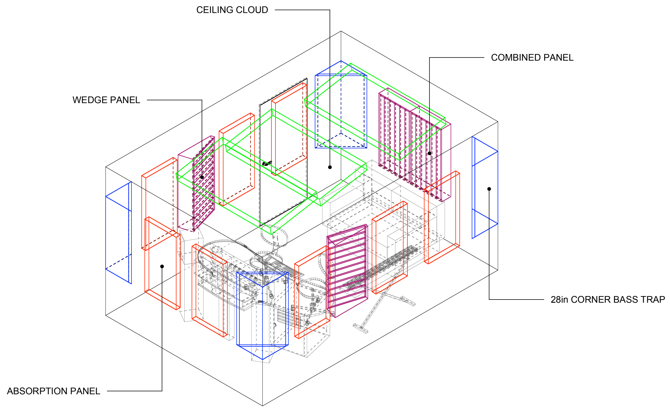
1 CONTROL ROOM KIT 150 - SAMPLE ROOM ISO VIEW 01.01 Scale: NTS
